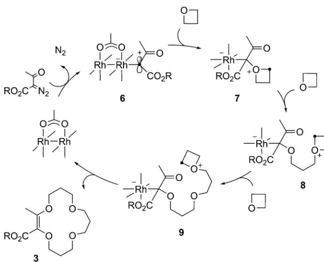
Scheme 2. Mechanistic rational. The electrophilic sites are indicated by dots.
